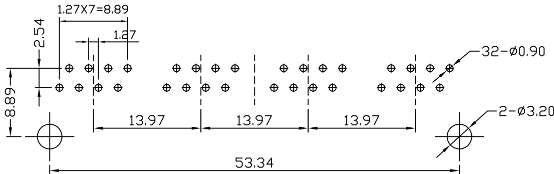
PC Board Layout (Top View)
